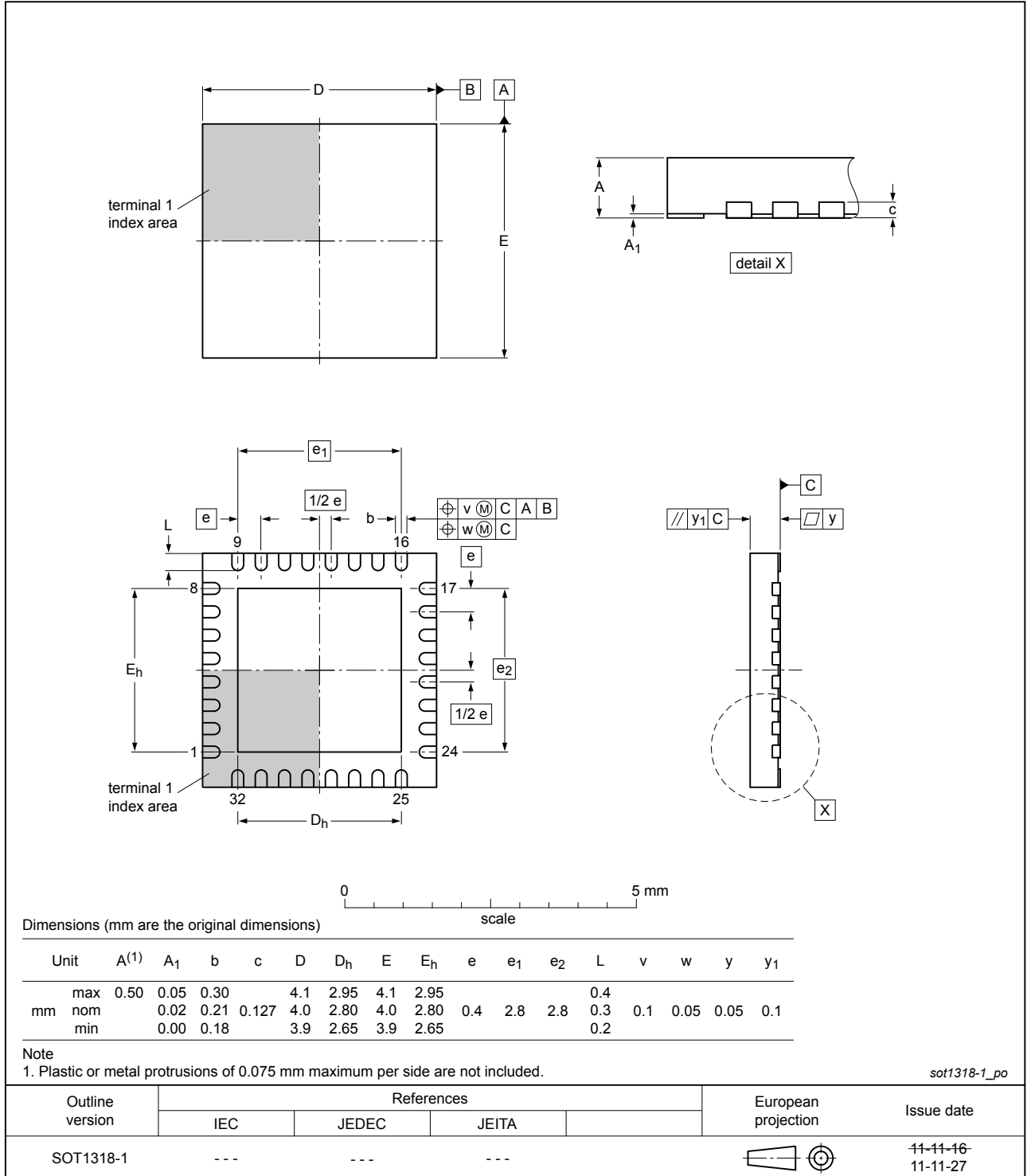
Fig. 1. Package outline HXQFN32 (SOT1318-1)
